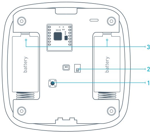
PICTURE 3. Battery compartment
